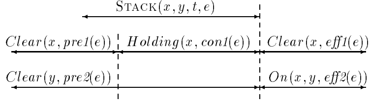
Figure 5: Necessary conditions for stacking x on y
